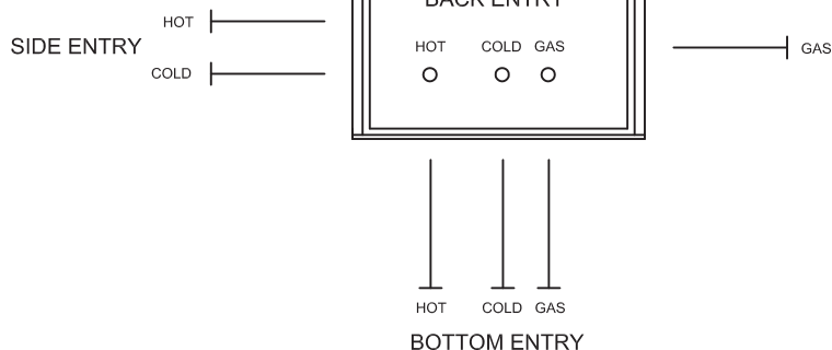
Figure 2: Piping options.
